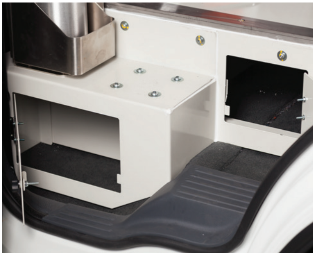
Under floor tools boxes
